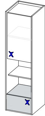
X-04 45 / 180 / 40
